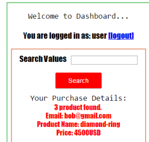
Figure 24: Attacker logged into application and doing an injection attack on search page
